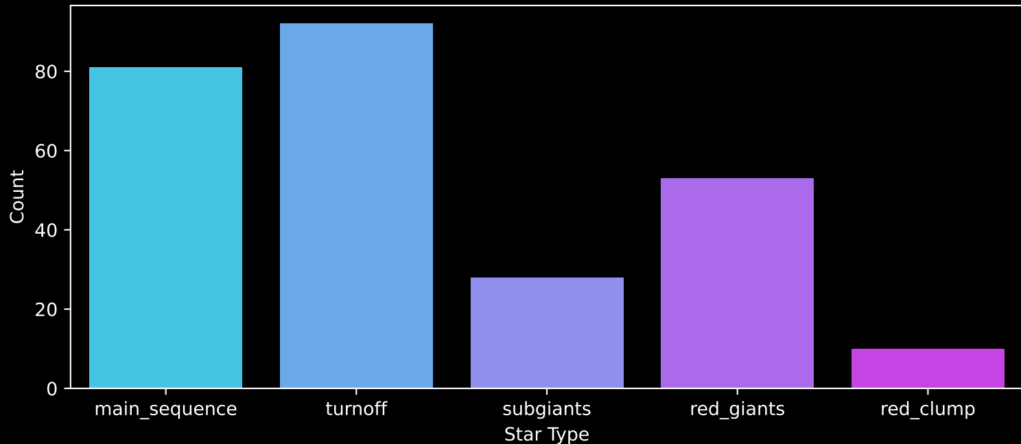
GALAH DR4 Field: [7143] Count plot of Star Type
