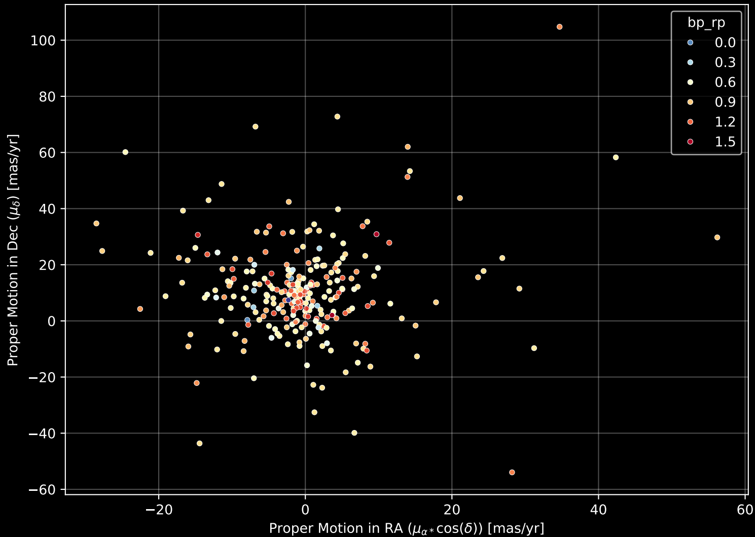
GALAH DR4 Field: [7143] Proper Motion Diagram (n= 264)
