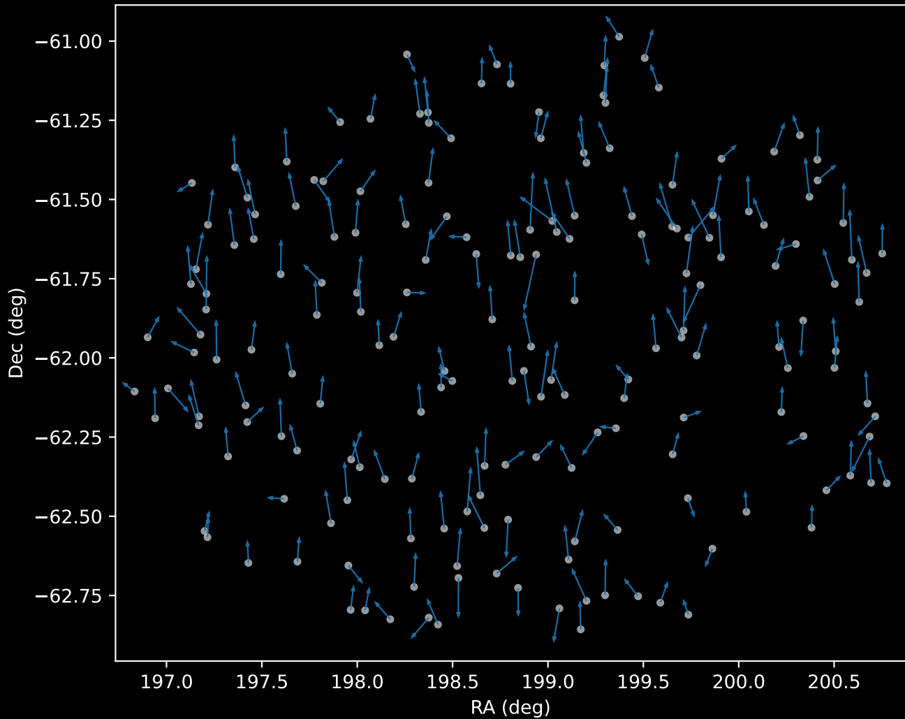
GALAH DR4 Cluster 0 Proper Motion Vectors (n=187)
