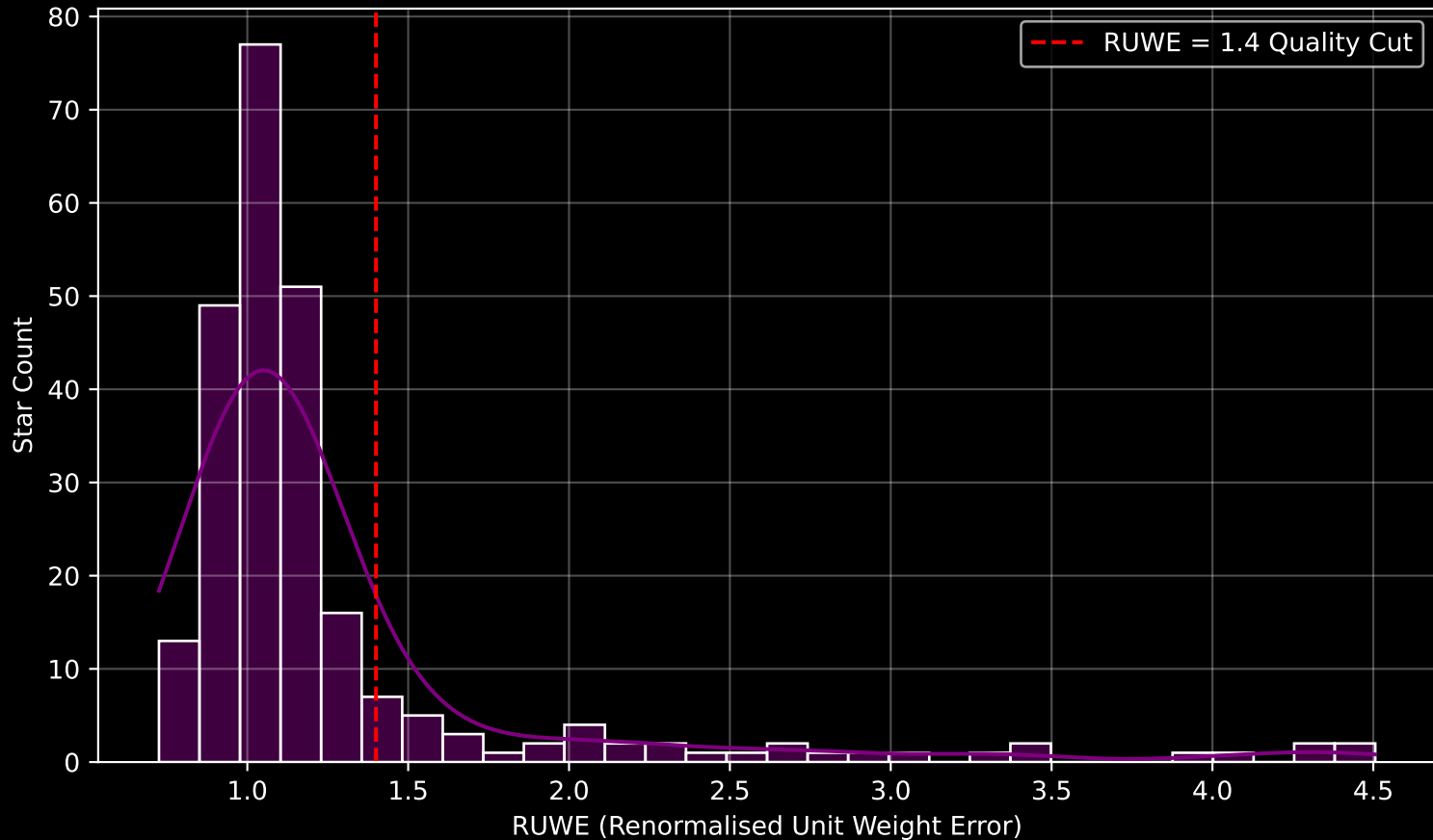
GALAH DR4 Field [7143] RUWE Distribution (n= 248)
